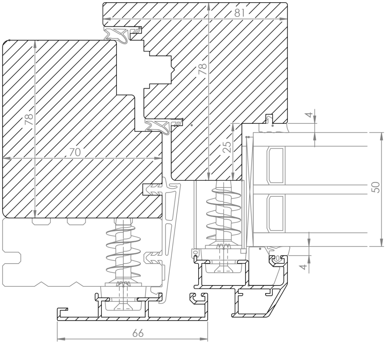
DETAIL D
