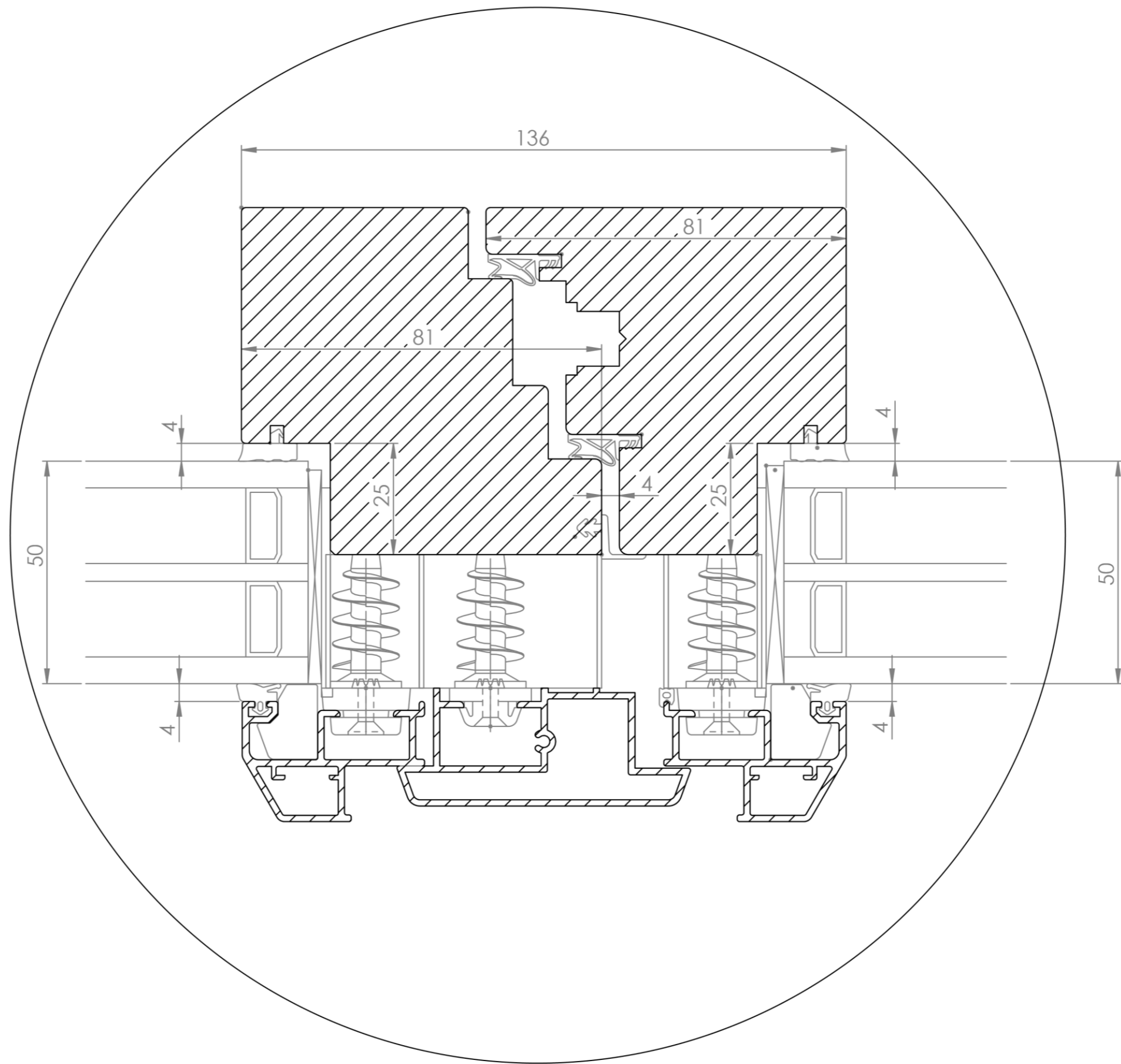
DETAIL E
